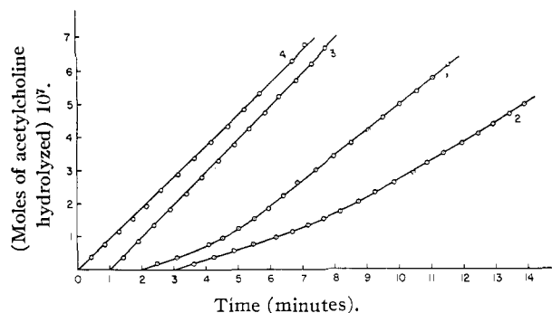
Fig. 1.—(1) Non-enzymatic hydrolysis of acetyluricine and (2) acetylbetonicine at 25.14^\circ , pH 7.1, and initial concentrations of 1.97 \times 10^{-3} M ; (3) enzymatic hydrolysis of acetyluricine and (4) of acetylbetonicine at pH 7.0 and 1.94 \times 10^{-3} M concentration.
